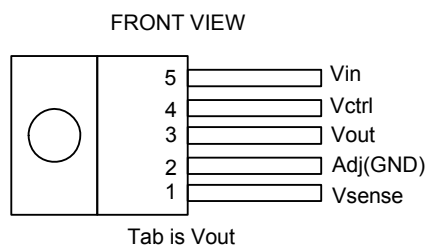
TO220-5L
