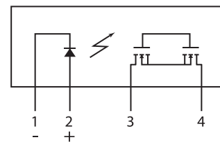
CPC1916Y Pinout
