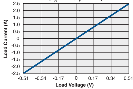
CPC1927 Typical Load Current vs. Load Voltage ( T_A = 25^\circ C, I_F = 10mA )
