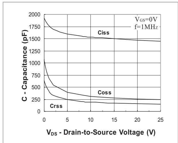
FIG.6- Capacitance
