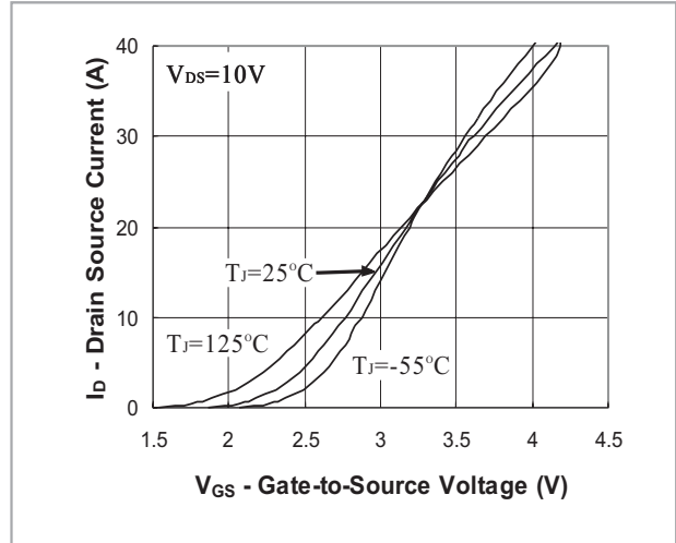
FIG.2- Transfer Characteristic
