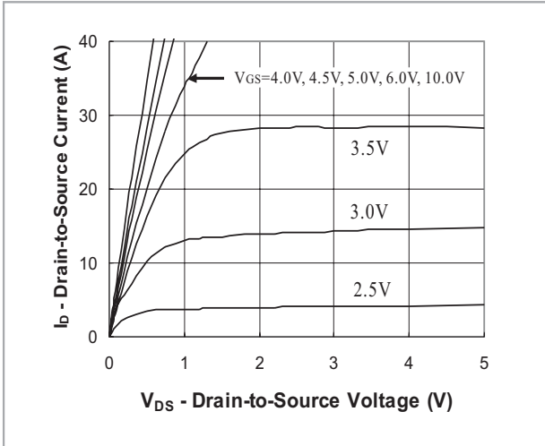
FIG.1- Output Characteristic
