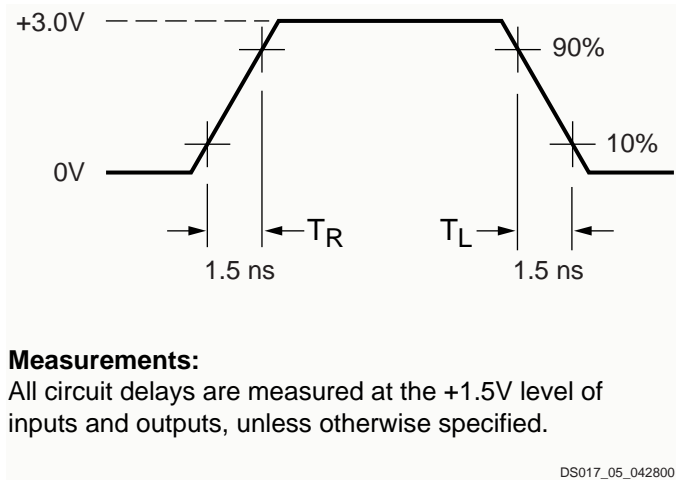
Figure 5: Voltage Waveform
