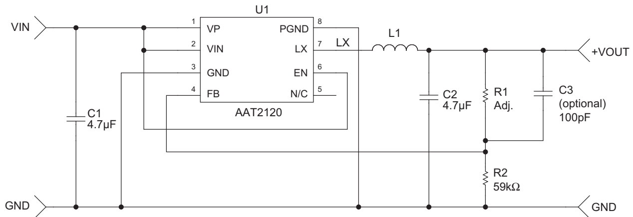
Figure 1: AAT2120 Schematic.
