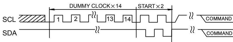
Fig.39-(a) DUMMY CLOCK x 14 + START + START
