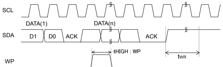
Fig.1-(e) WP Timing Of The Write Cancel Operation
