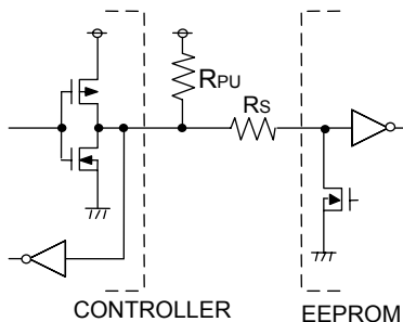
Fig.44 I/O Circuit
