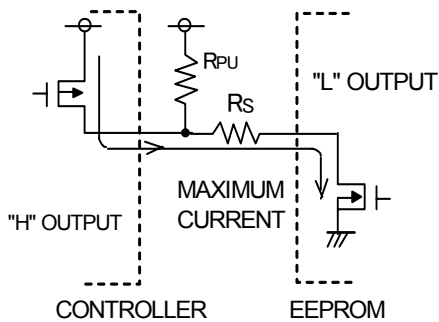
Fig.47 I/O Circuit
