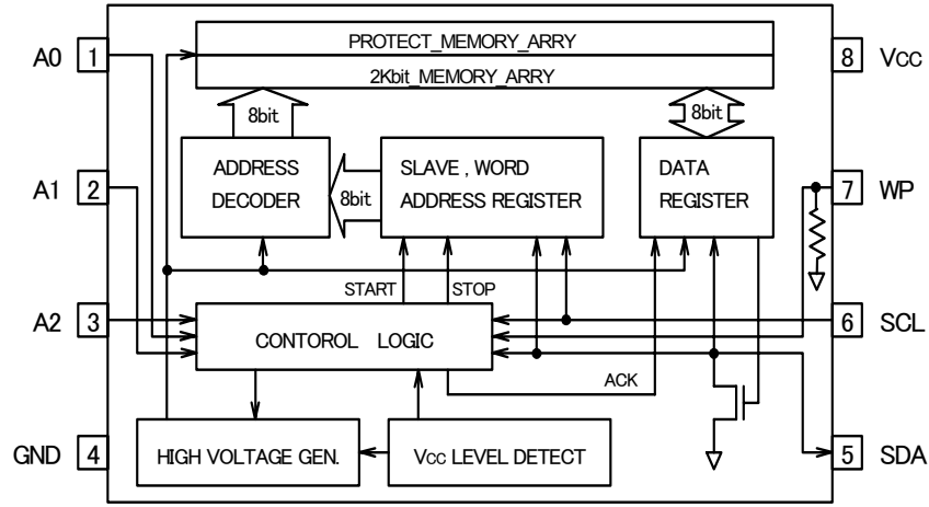
Fig.2 Block Diagram
