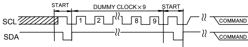
Fig.39-(b) START + DUMMY CLOCK x 9 + START
