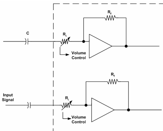
Figure 38. Input Resistor
