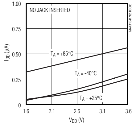
V DD SHUTDOWN SUPPLY CURRENT vs. VOLTAGE
