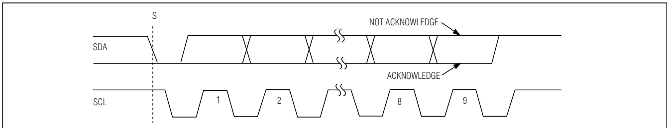
Figure 8. Acknowledge Bits
