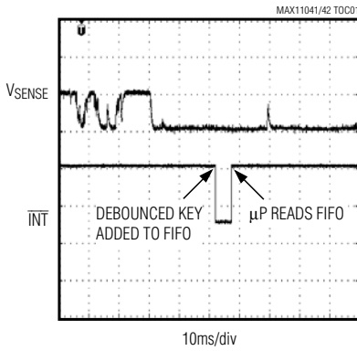
DEBOUNCE SCOPE SHOT (FALLING)
