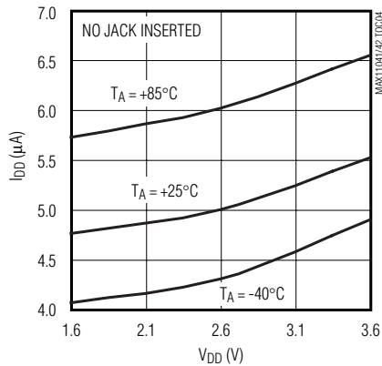
V DD SUPPLY CURRENT vs. VOLTAGE
