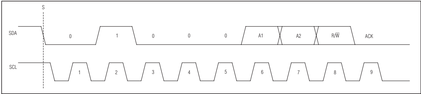
Figure 6. Slave Address and R/W Bit
