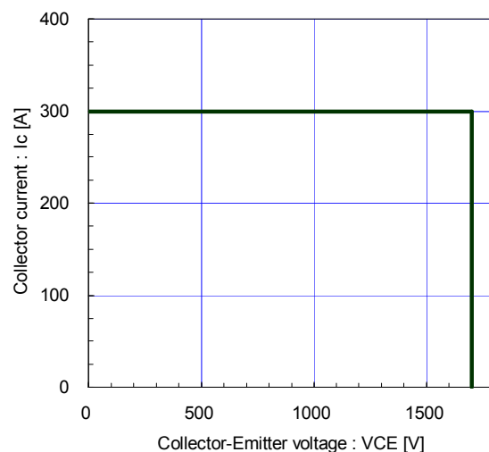
Reverse bias safe operating area (max.) +V_{GE}=15V , -V_{GE} \leq 15V , R_g \geq 3.3\Omega , T_j \leq 125^\circ C
