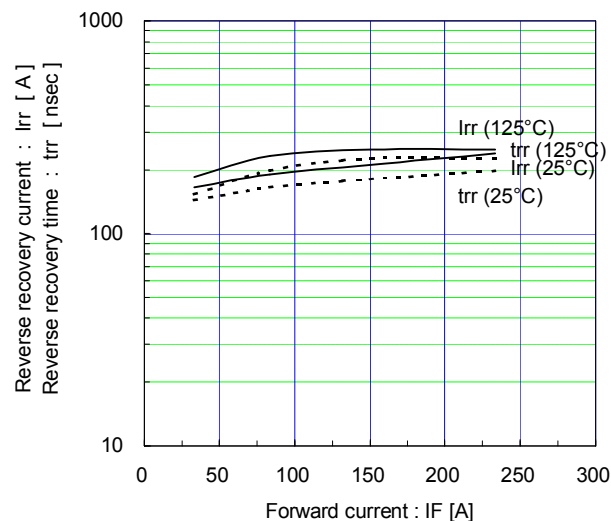
Reverse recovery characteristics (typ.) V_{CC}=900V , V_{GE}=\pm 15V , R_g=3.3\Omega
