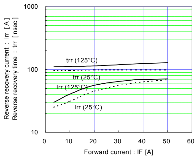
[ Inverter ] Reverse recovery characteristics (typ.) V_{cc}=600V , V_{GE}=\pm 15V , R_g=33\Omega
