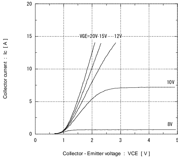
[ Brake ] Collector current vs. Collector-Emitter voltage T j = 25°C (typ.) / chip
