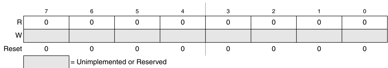
Figure 25-24. Flash Reserved1 Register (FRSV1)
