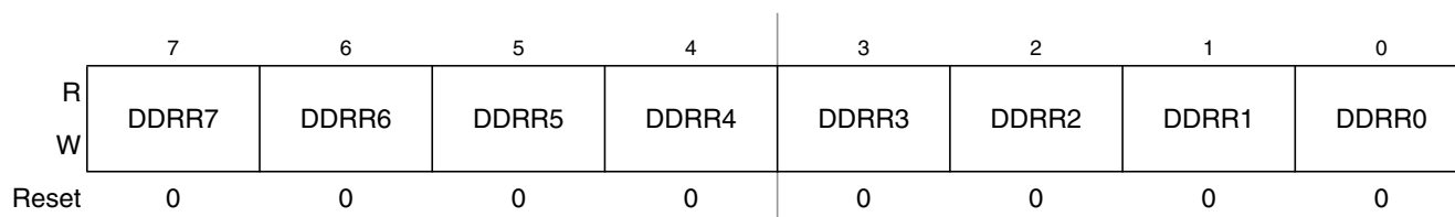
Figure 2-85. Port R Data Direction Register (DDRR)
