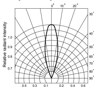
Fig.6 Radiation diagram
