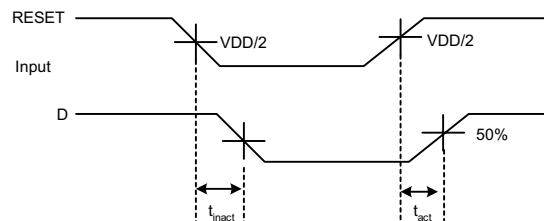
Figure 4. Active and Inactive Times
