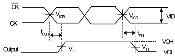
Figure 7. Propagation Delay
