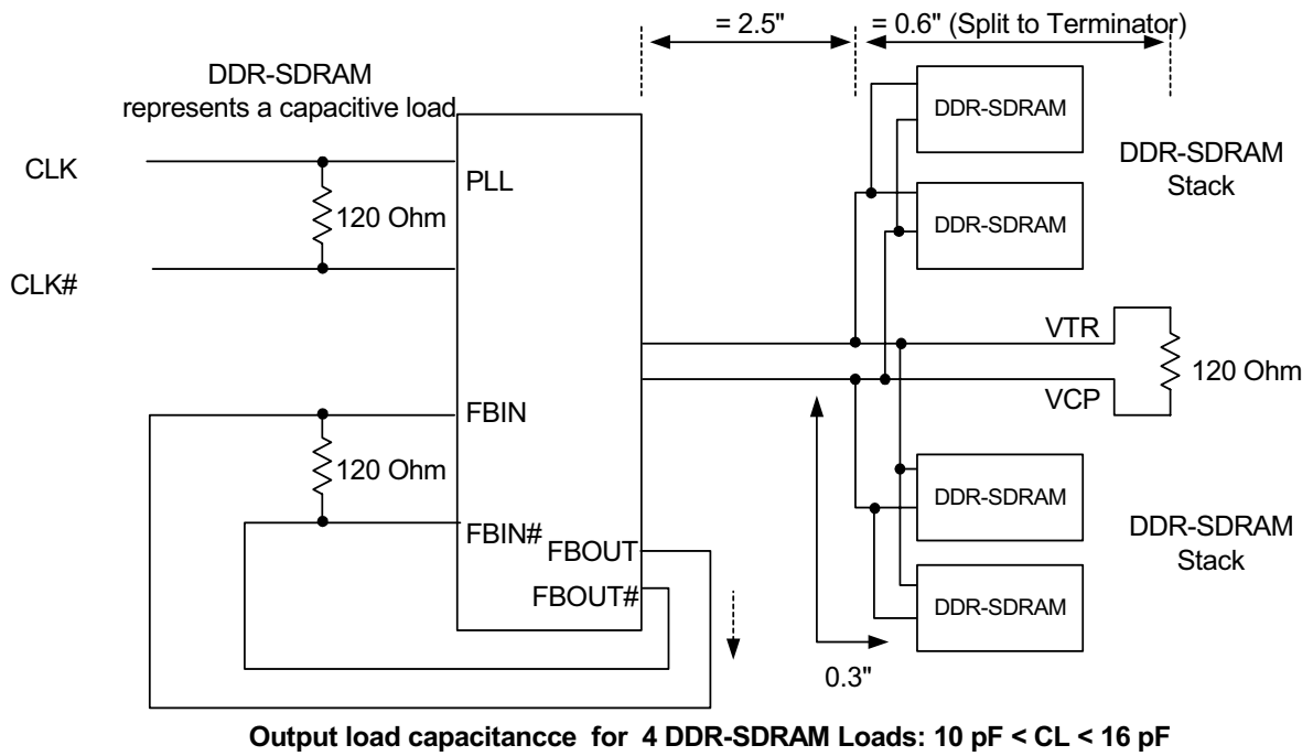
Figure 5. Clock Structure # 1
