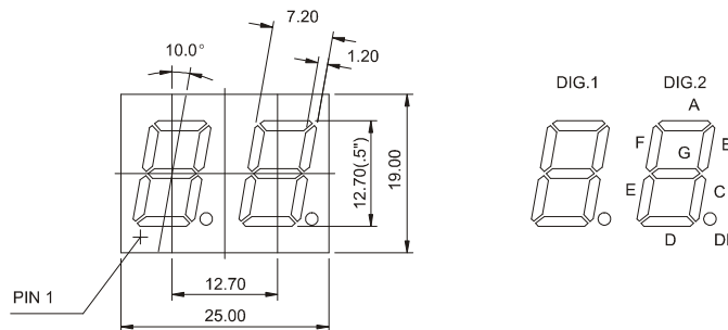
FYD-5021 Series
