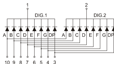
FYD-5021Gx
