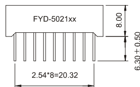
FYD-5021Gx
