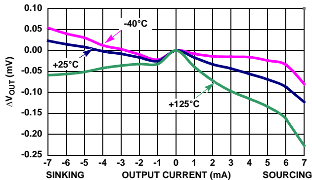
FIGURE 48. LOAD REGULATION
