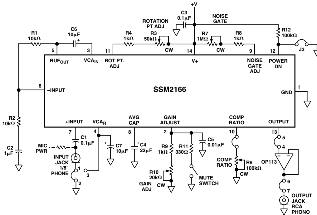
Figure 12. Evaluation Board
