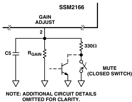
Figure 9. Details of SSM2166 Mute Option
