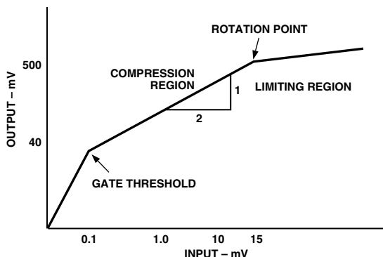
Figure 15. Transfer Characteristic
