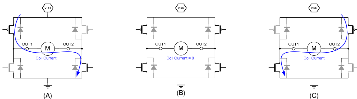
Soft Switching Output Voltages
