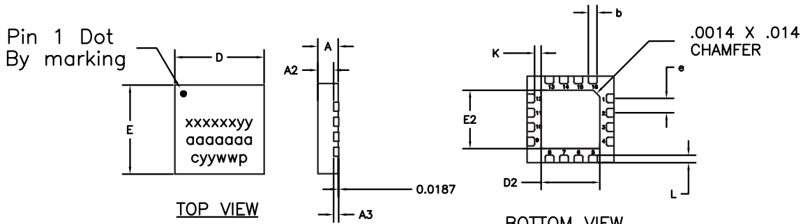
BOTTOM VIEW
