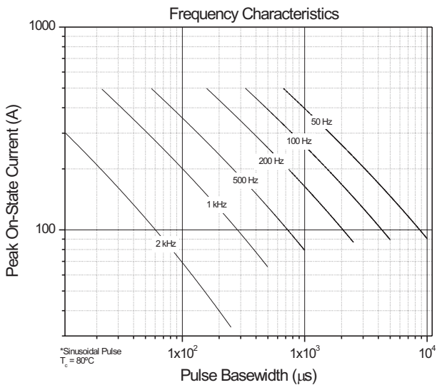
Fig. 9 - Frequency Characteristics
