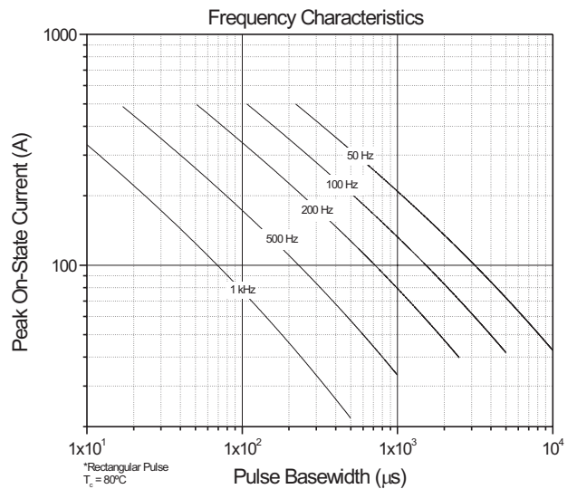
Fig. 10 - Frequency Characteristics
