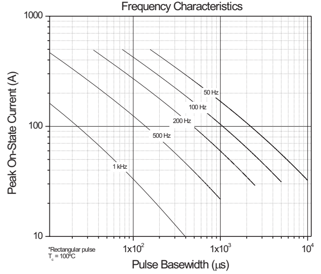
Fig. 12 - Frequency Characteristics
