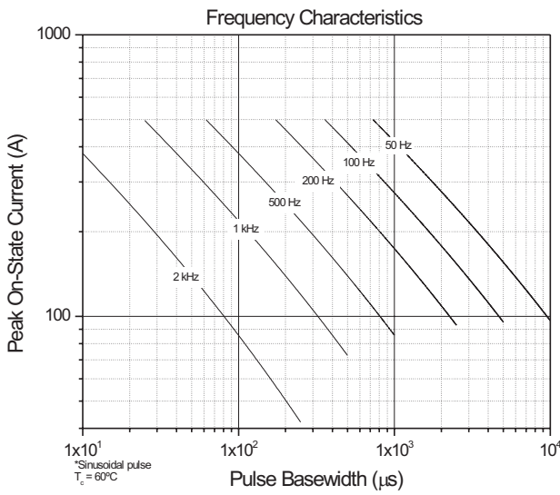
Fig. 7 - Frequency Characteristics
