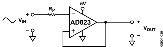
Figure 39. AD823 Input Response: V_{IN} = 0 to +V_S + 200 mV, V_{OUT} = 0 to +V_S , R_P = 49.9 k \Omega
