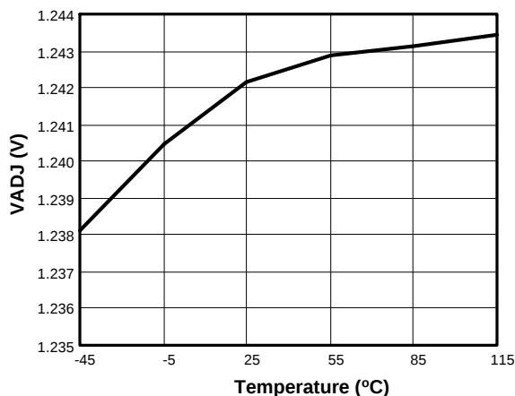
AME8844BEQA VADJ vs. Temperature
