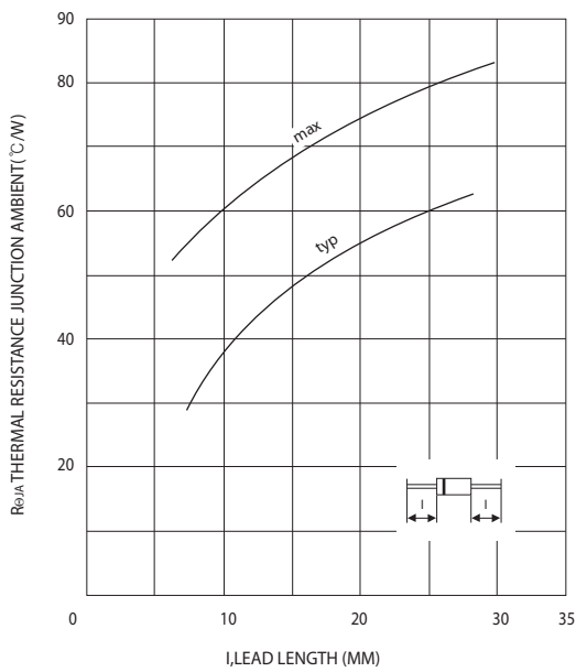
FIG.3-TYPICAL THERMAL IMPEDANCE
