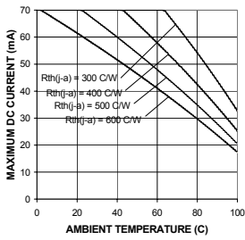
Figure 3. HPWT-xx00 Maximum DC Forward Current vs. Ambient Temperature.
