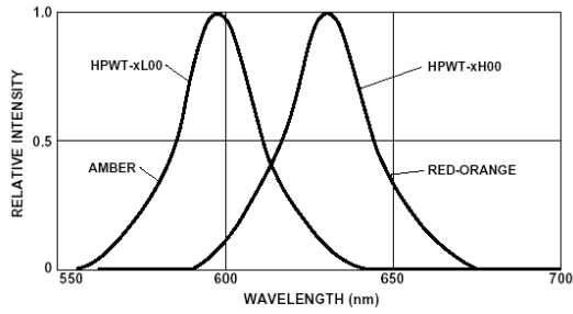
Figure 1. Relative Intensity vs. Wavelength.
