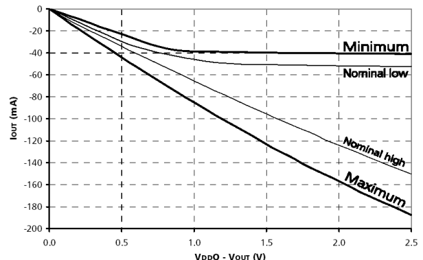
Figure 10: Pull-Up Characteristics
