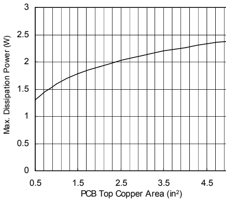
SOT-89 Max. Power Dissipation vs. PCB Top Copper Area T_{AMB} = 25^{\circ}\text{C} ; Still Air
