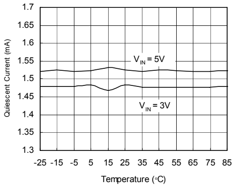
Quiescent Current vs. Temperature(G965-15)
