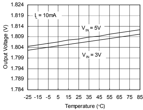
Output Voltage vs. Temperature(G965-18)
