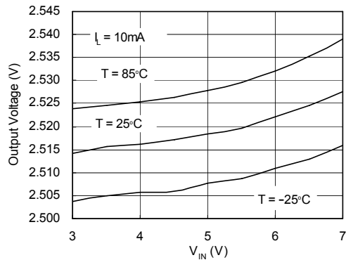
Output Voltage vs. VIN(G965-25)
