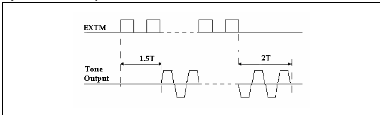
Figure 2. EXTM timings
