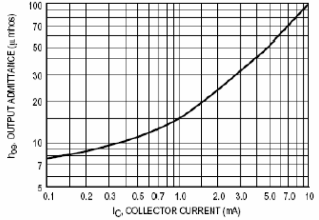
Figure 8 Output Admittance
