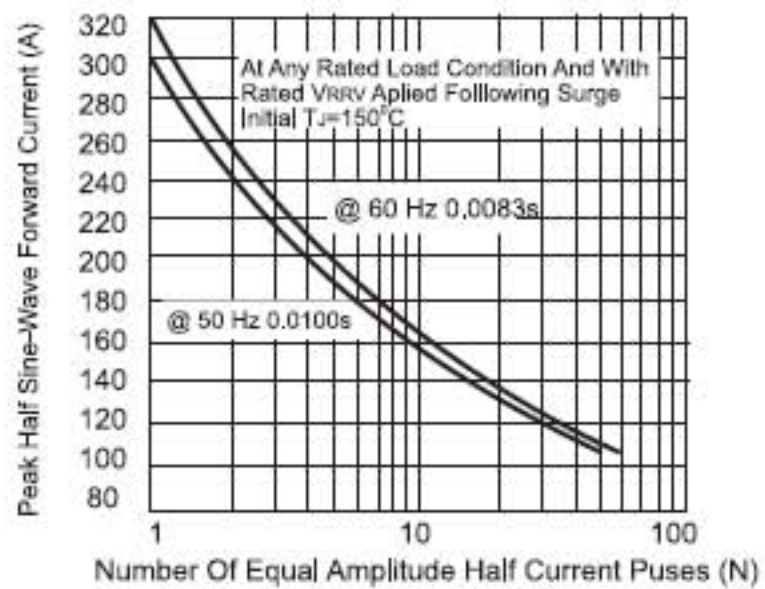
FIG.4 - Maximum Non-Repetitive Surge Current
