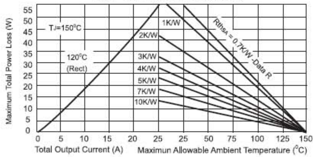
FIG.3 - Total Power Loss Characteristics
