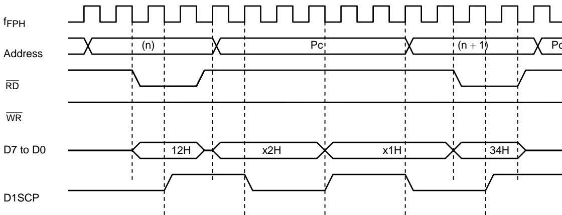
Figure 3.14.9 Byte Read and Nibble Write Timing
