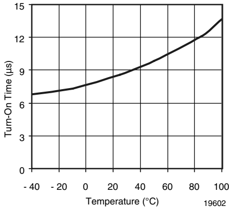
Fig. 8 - Turn-On Time vs. Temperature
