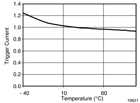
Fig. 5 - Normalized Trigger Current vs. Temperature
