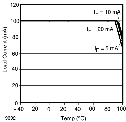
Fig. 1 - On-State Load Current vs. Temperature
