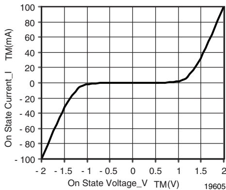
Fig. 4 - On-State Current vs. VTM
