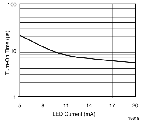
Fig. 6 - Turn-On Time vs. LED Current
