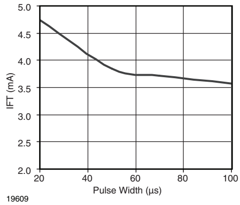
Fig. 9 - Trigger Current vs. Pulse Width
