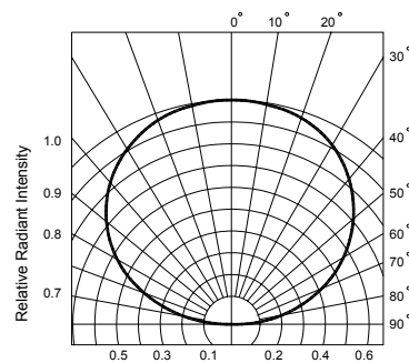
RADIATION DIAGRAM
