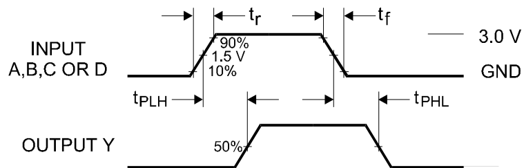
Figure 1. Switching Waveforms
