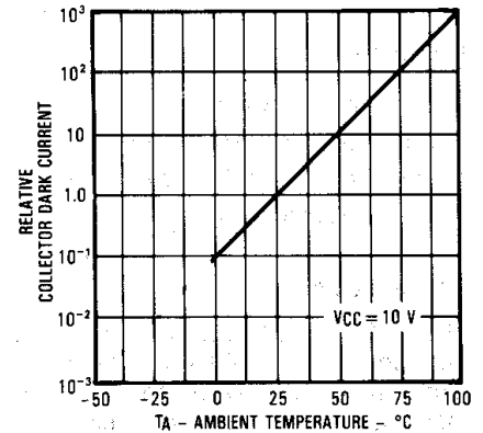
Relative Collector Dark Current vs Ambient Temperature
