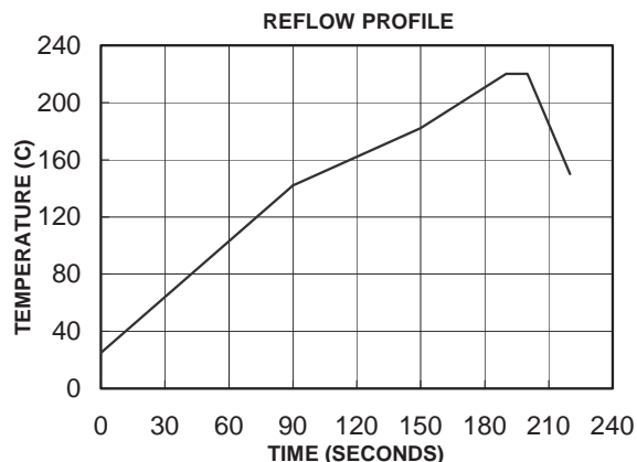
Figure 17 VPOL10A-12W-SMT Reflow Profile
