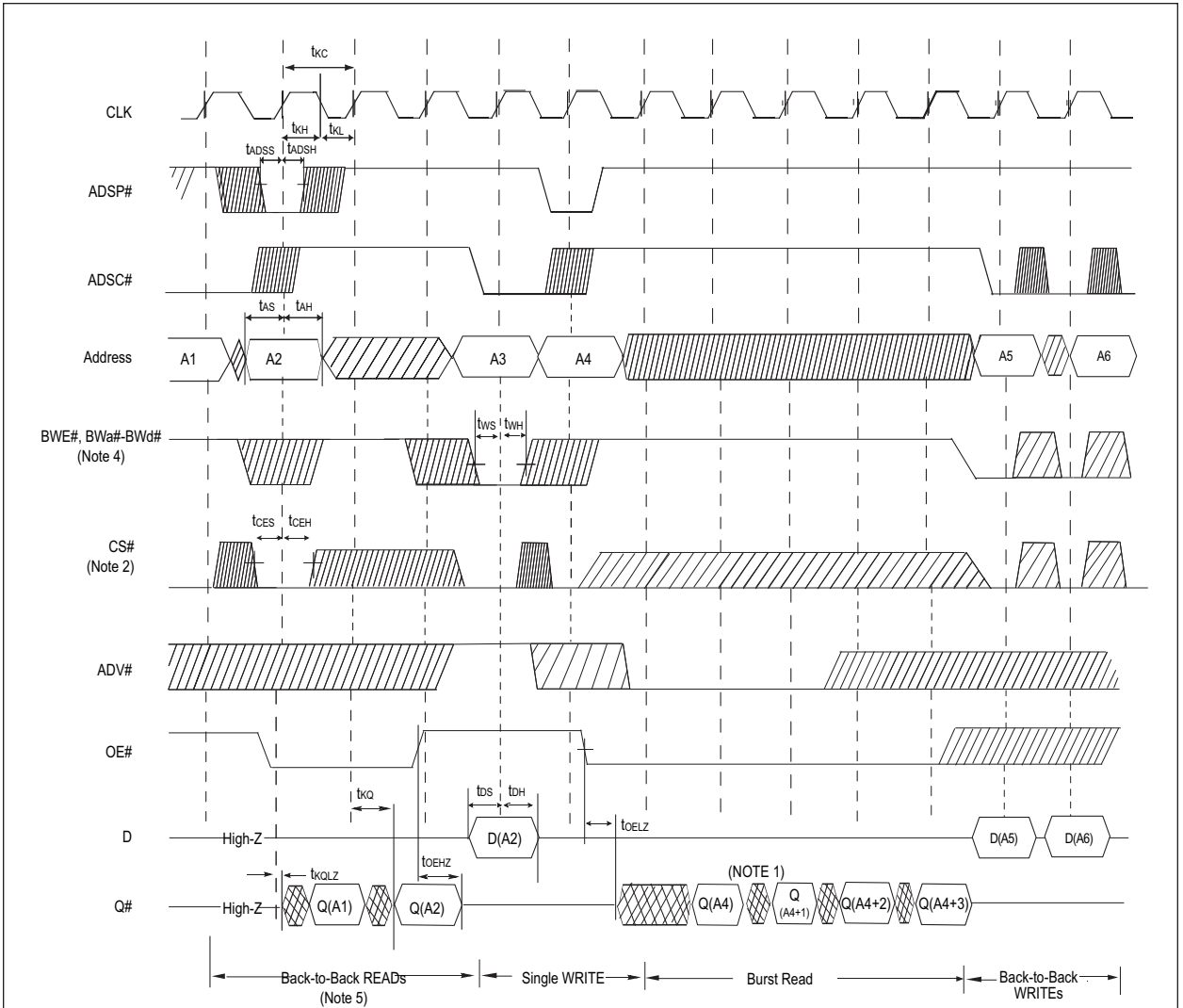
FIGURE 5 – READ/WRITE TIMING 3
