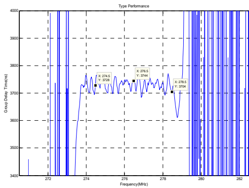
Group Delay Variation (f0±2MHz)
