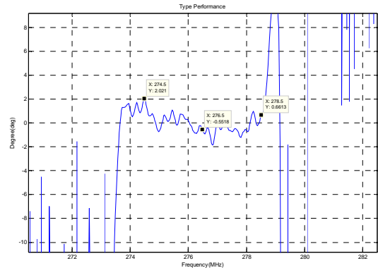
Phase Linearity (f0±2MHz)
