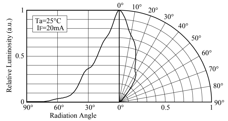
■ Directivity (NSPG520S)
