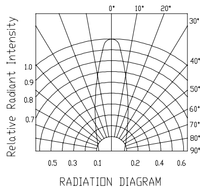
Radiation Diagram T a =25°
