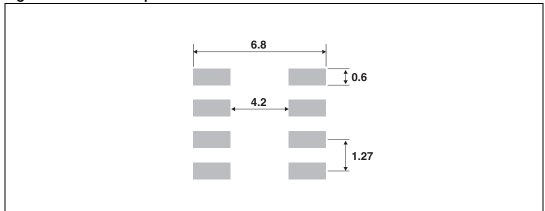
Figure 18. SO-8 Footprint
