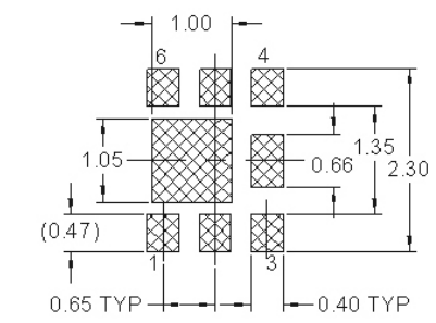
RECOMMENDED LAND PATTERN OPT 2
