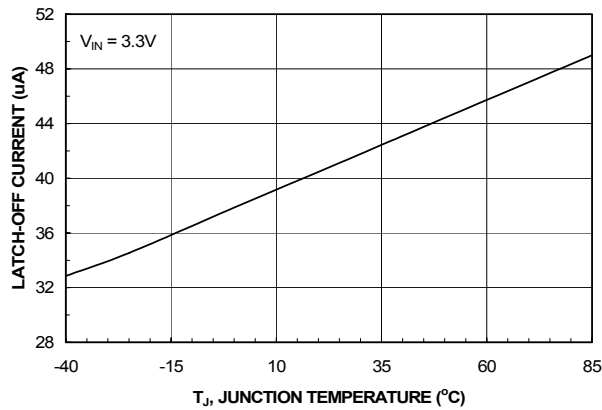
Figure 5. I_{LATCLOFF} vs. Temperature
