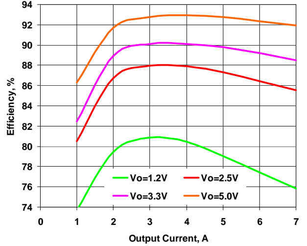
Figure 4. Efficiency vs. Load. Vin=9.6V, Fsw=500kHz
