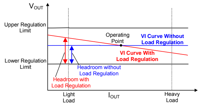
Figure 27. Optimal Voltage Positioning Concept
