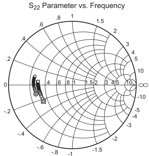
Condition: V_{CE} = 3.3\text{ V} , Z_0 = 50\ \Omega 400 to 3000 MHz (100 MHz Step) ○ ( I_C = 100\text{ mA} ) □ ( I_C = 250\text{ mA} )
