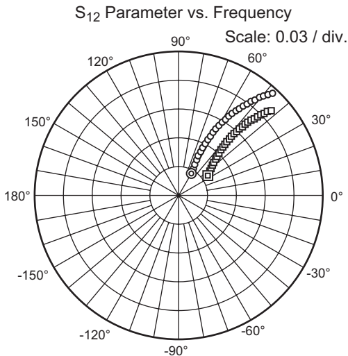
Condition: V_{CE} = 3.3\text{ V} , Z_0 = 50\ \Omega 400 to 3000 MHz (100 MHz Step) ○ ( I_C = 100\text{ mA} ) □ ( I_C = 250\text{ mA} )
