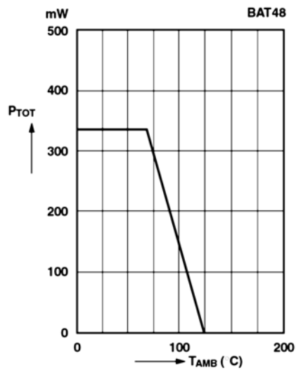
Admissible Power Dissipation vs. Ambient Temperature
