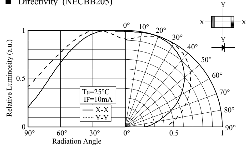
■ Directivity (NECBB205)
