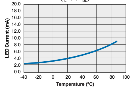
CPC1978 Typical I_F for Switch Operation vs. Temperature ( I_L=0.5A_{DC} )
